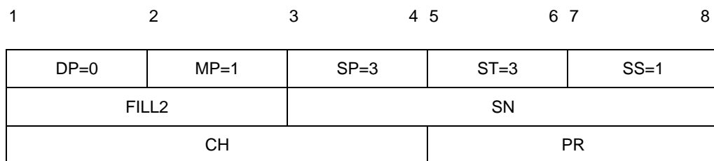
Figure 5-14. REJECT packet
