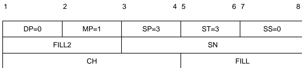
Figure 5-13. INTERRUPT CONFIRMATION packet
