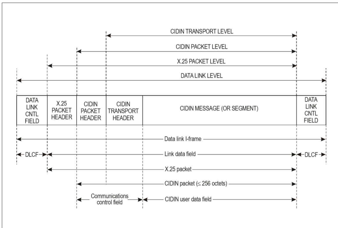
Figure 8-2. CIDIN terminology
