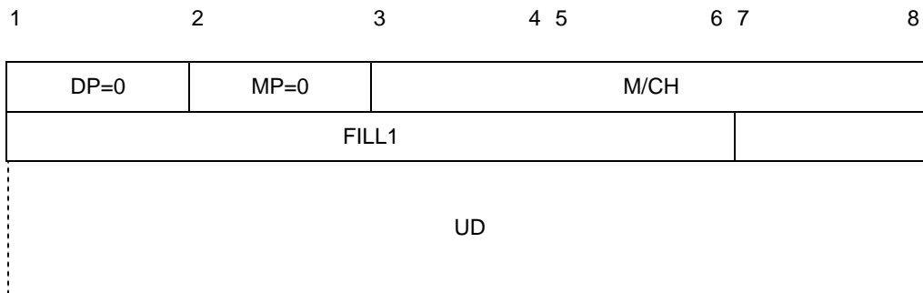
Figure 5-21. SHORT FORM MSP packet
