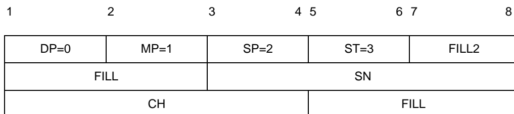
Figure 5-18. RESET CONFIRMATION packet
