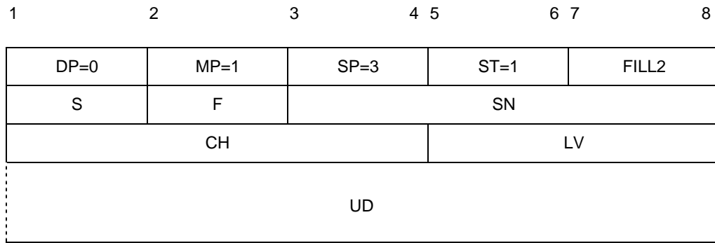
Figure 5-12. INTERRUPT packet
