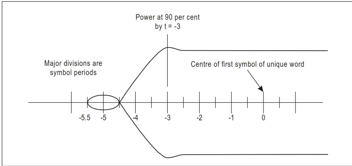
Figure 6-1. Transmitter power stabilization
