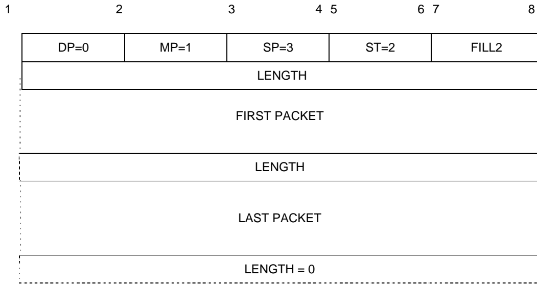
Figure 5-20. MULTIPLEX packet
