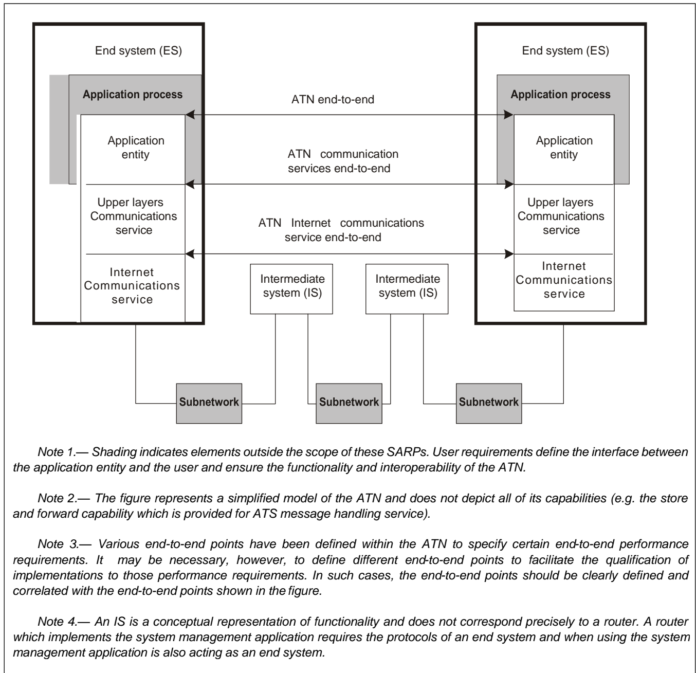
Figure 3-1 Conceptual model of the ATN
