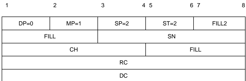
Figure 5-17. RESET REQUEST packet
