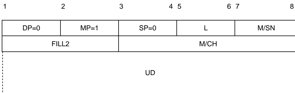
Figure 5-22. LONG FORM MSP packet
