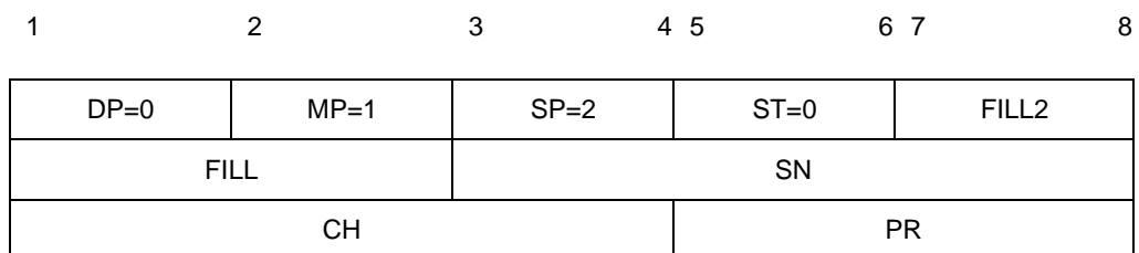
Figure 5-15. RECEIVE READY packet
