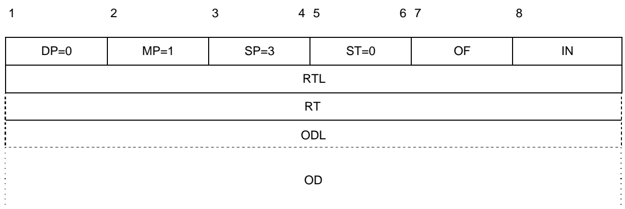
Figure 5-19. ROUTE packet
