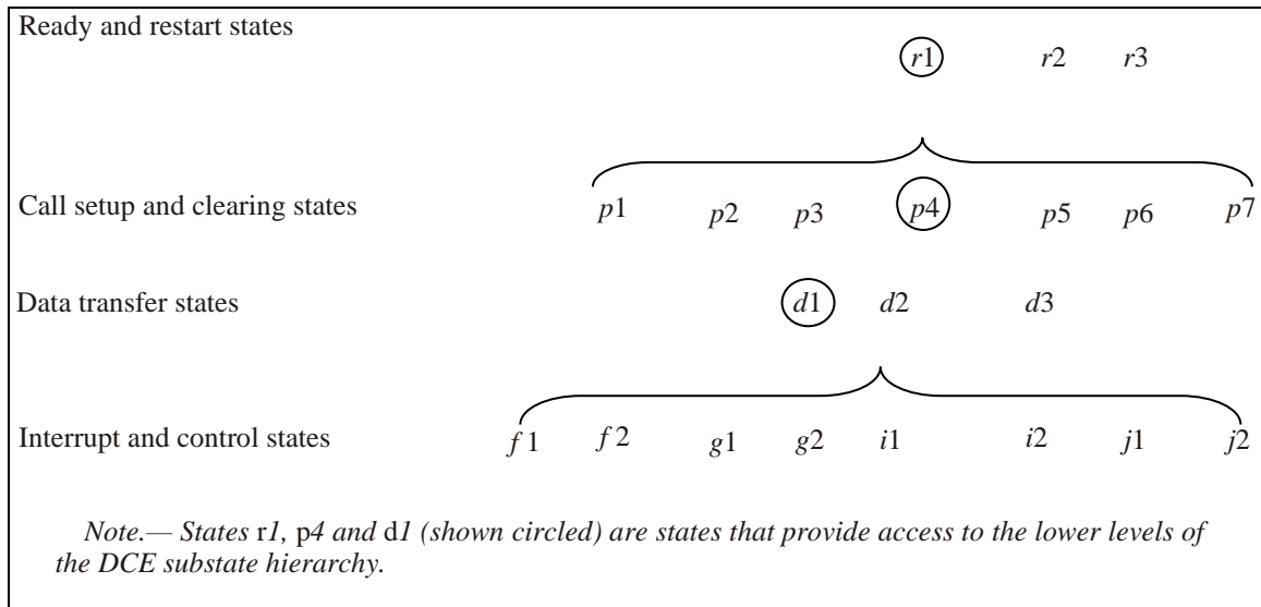
Figure 5-2. DCE substate hierarchy
