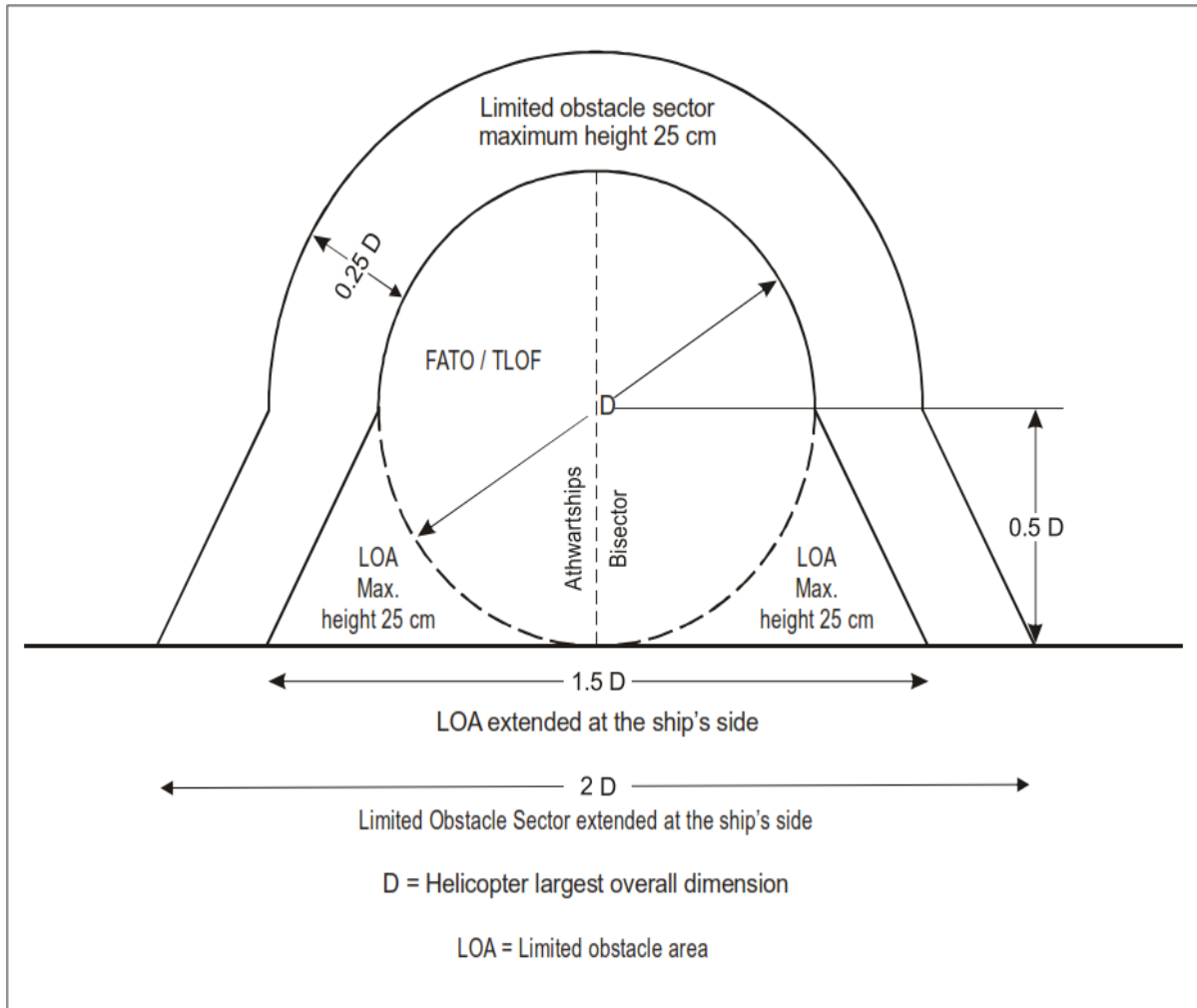
Figure 4-11. Ships-side non-purpose-built heliport obstacle limitation sectors and surfaces
