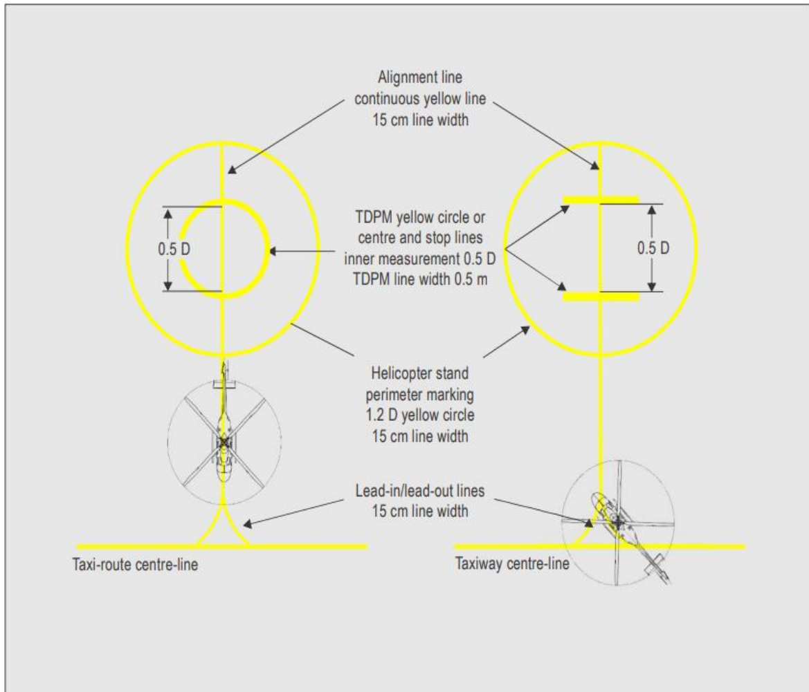
Figure 5-9. Helicopter stand markings
