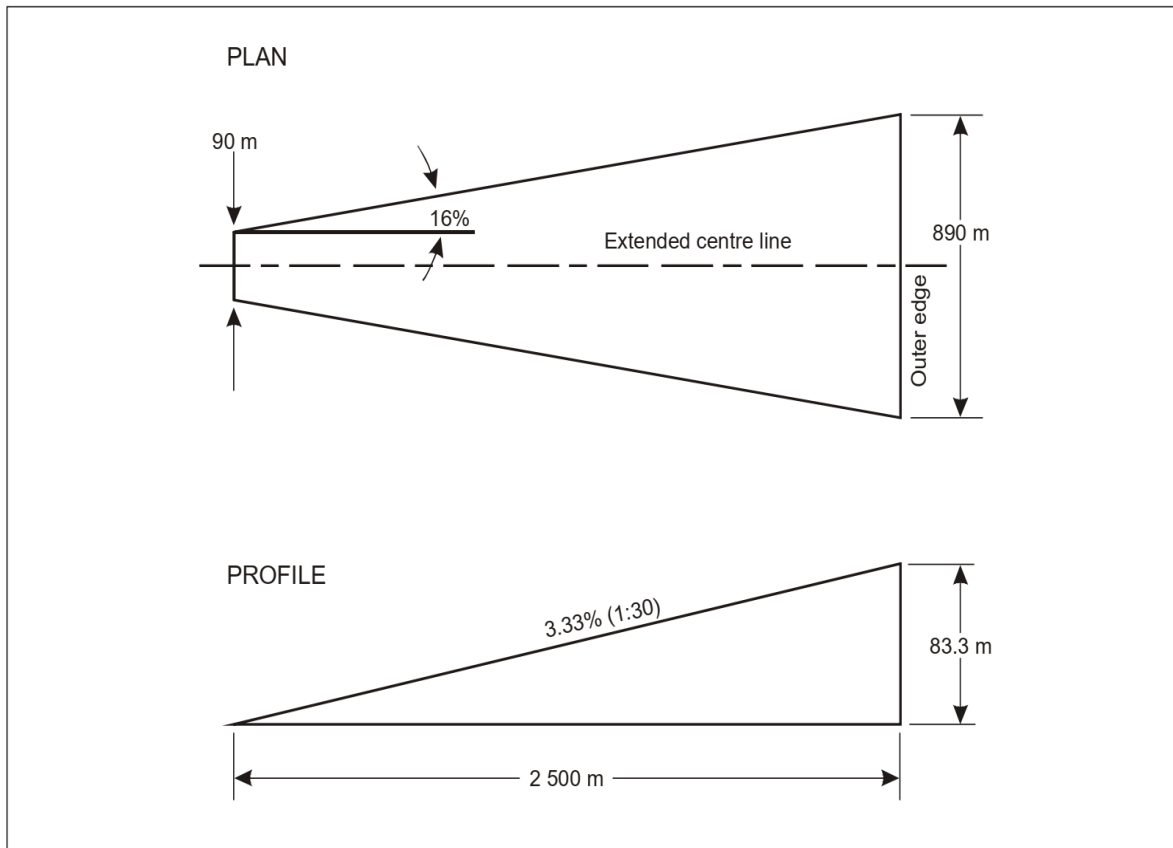
Figure A-4. Approach surface for non-precision approach FATO
