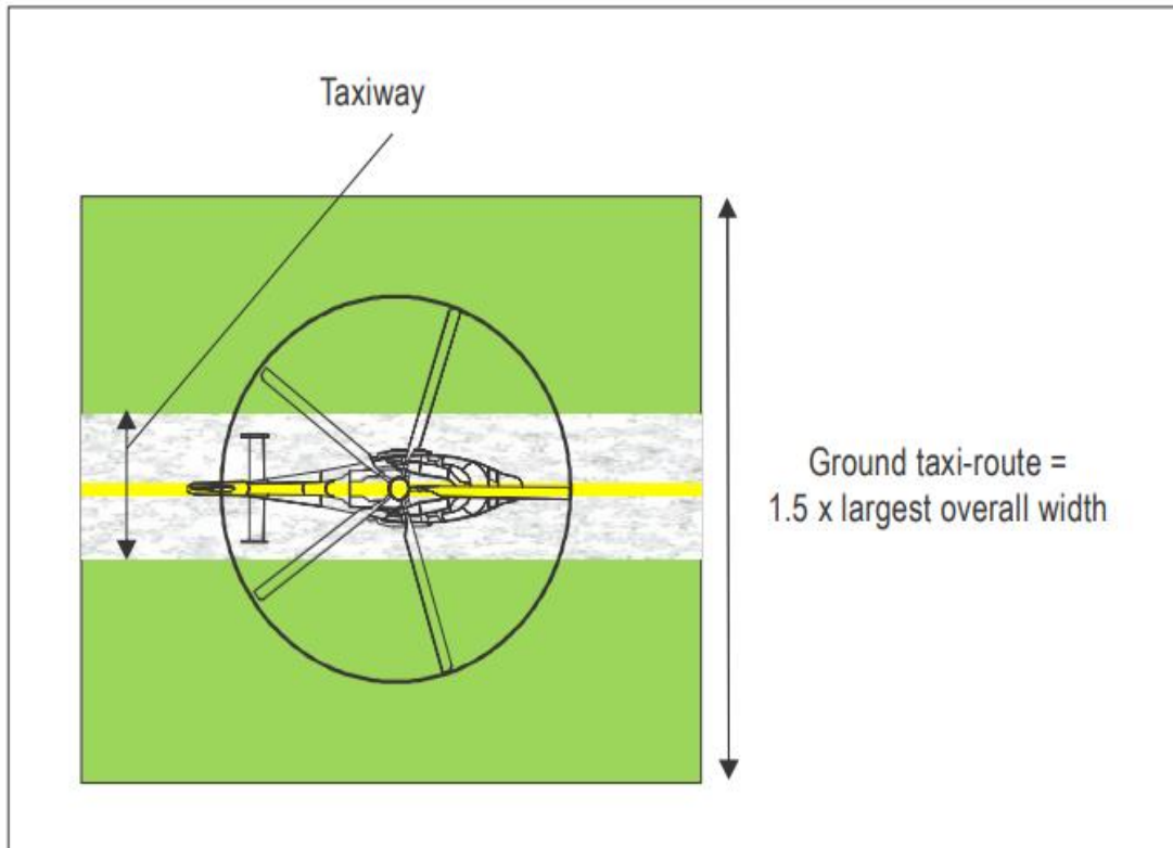
Figure 3-3. Helicopter taxiway/ground taxi-route
