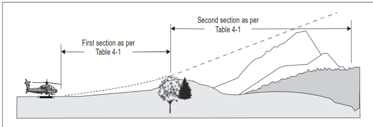
b) Approach and take-off climb surfaces - "B" slope profile - 8% and 16% design
