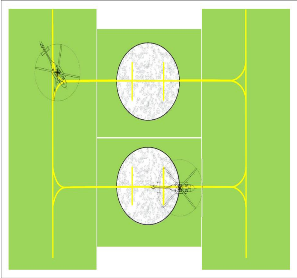
Figure 3-7. Air taxi-through stands (with air taxi-route) simultaneous use
