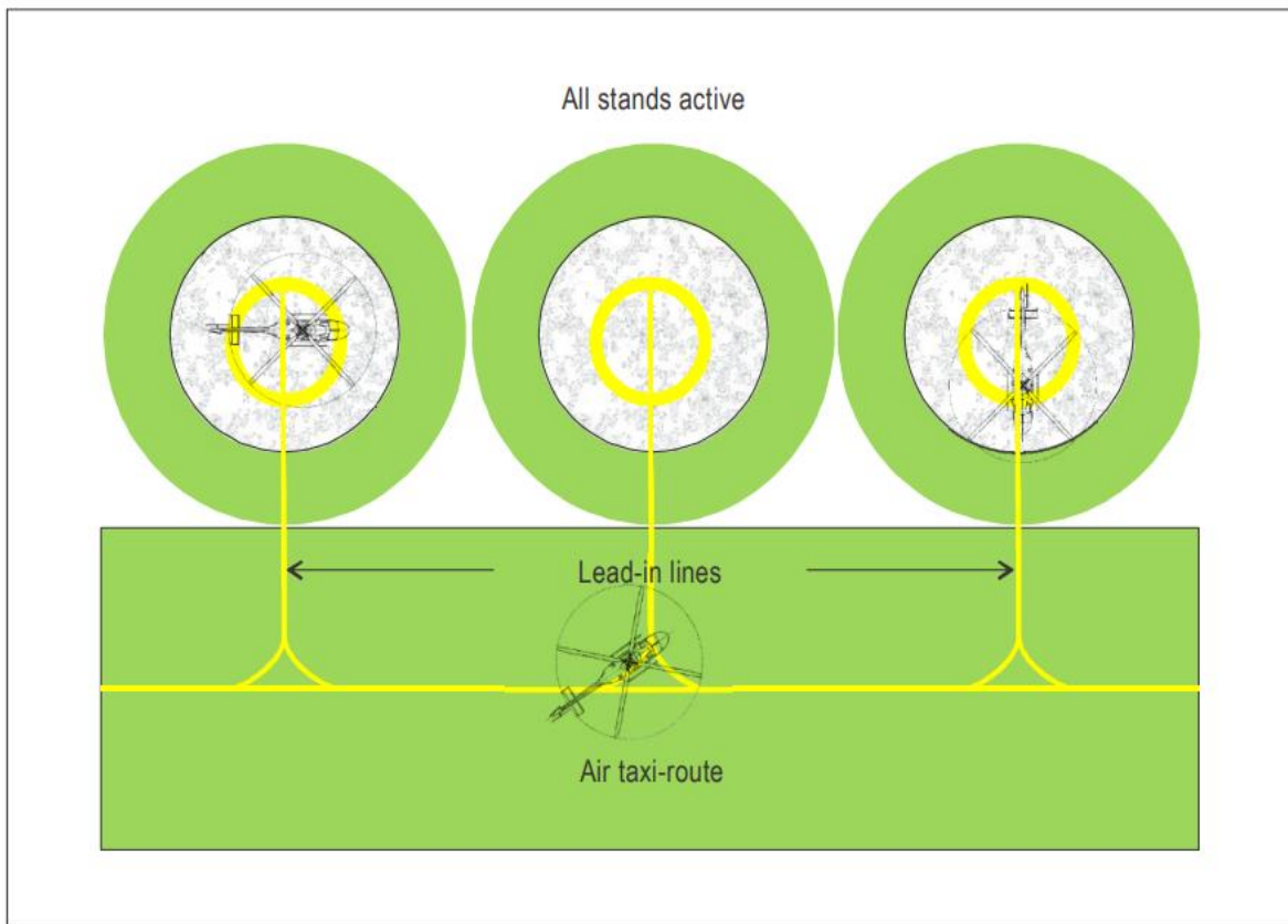
Figure 3-5. Turning stands (with air taxi-routes) — simultaneous use
