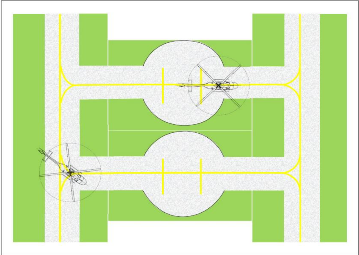
Figure 3-6. Ground taxi-through stands (with taxiway/ground taxi-route) simultaneous use
