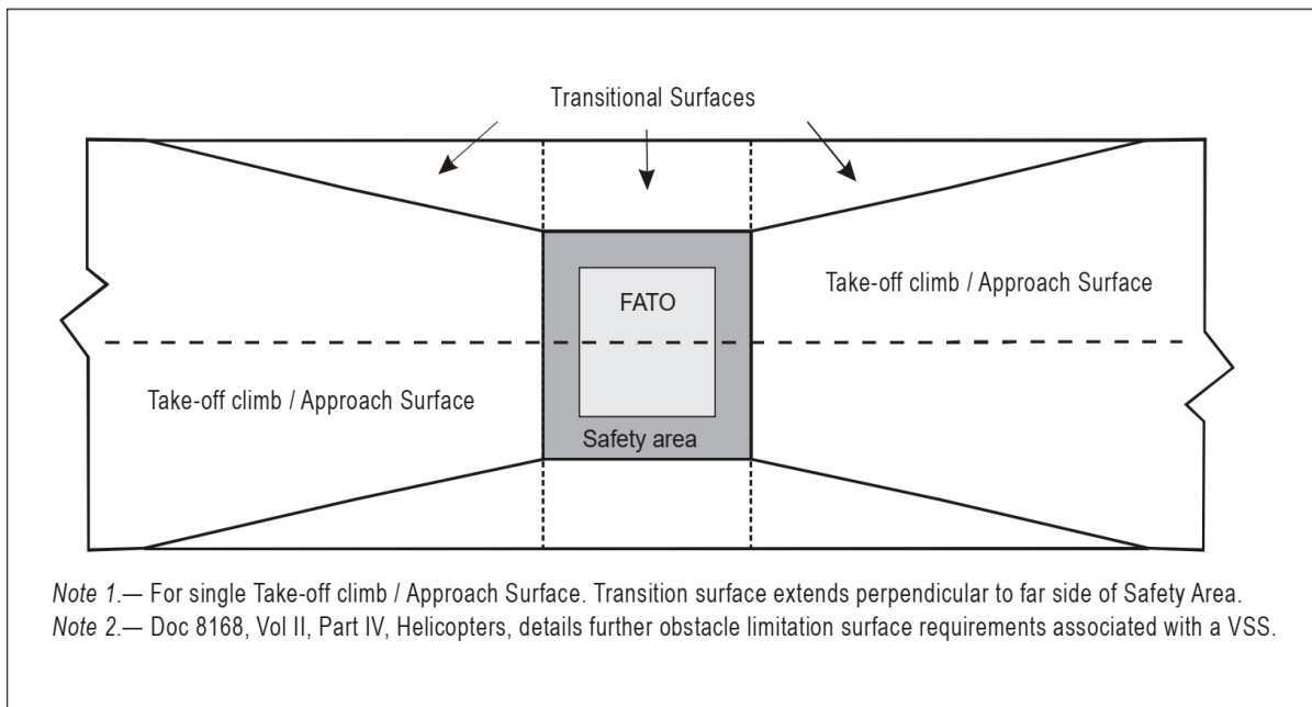
Figure A-5. Transitional surfaces for an instrument FATO with a non-precision and/or precision approach
