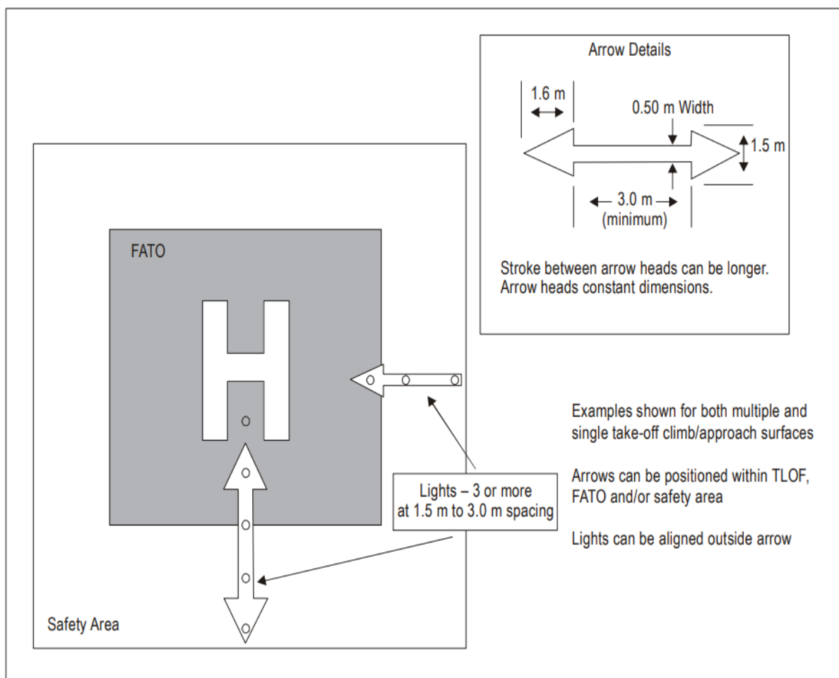
Figure 5-10. Flight path alignment guidance markings and lights
