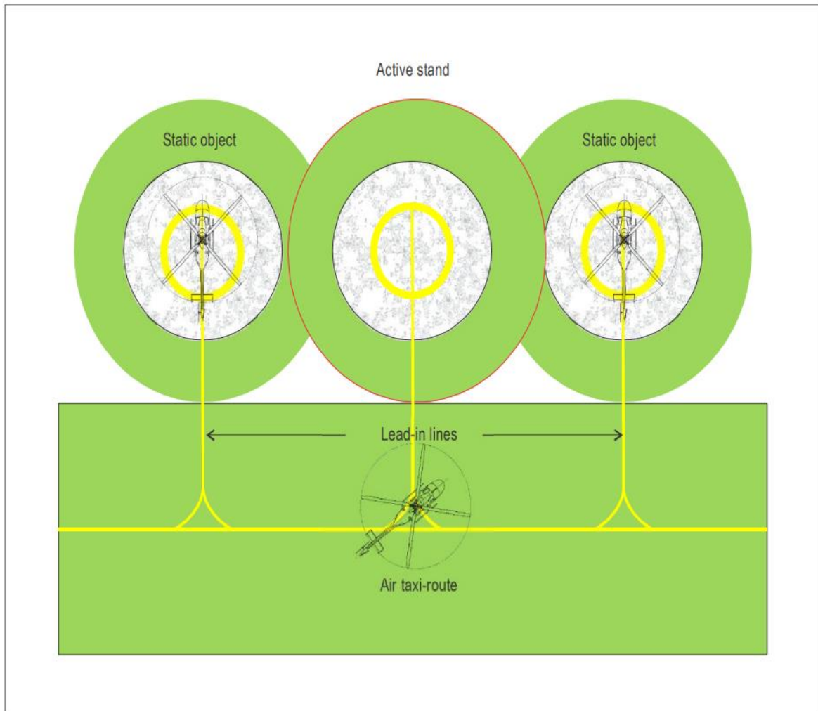
Figure 3-9. Turning stands (with air taxi-route) non-simultaneous use — inner stand active
