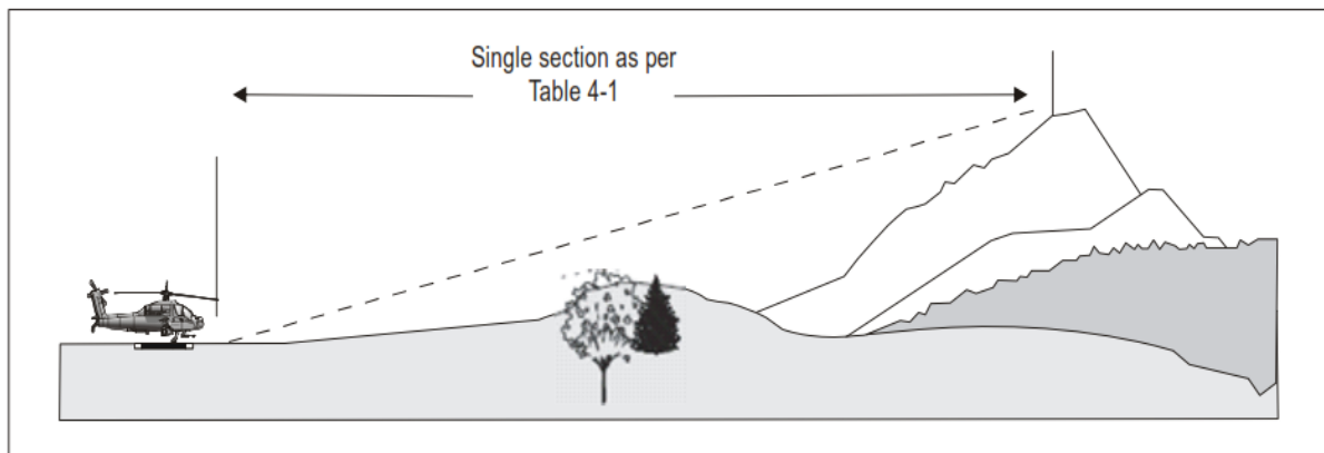
c) Approach and take-off climb surfaces - "C" slope profile - 12.5% design
