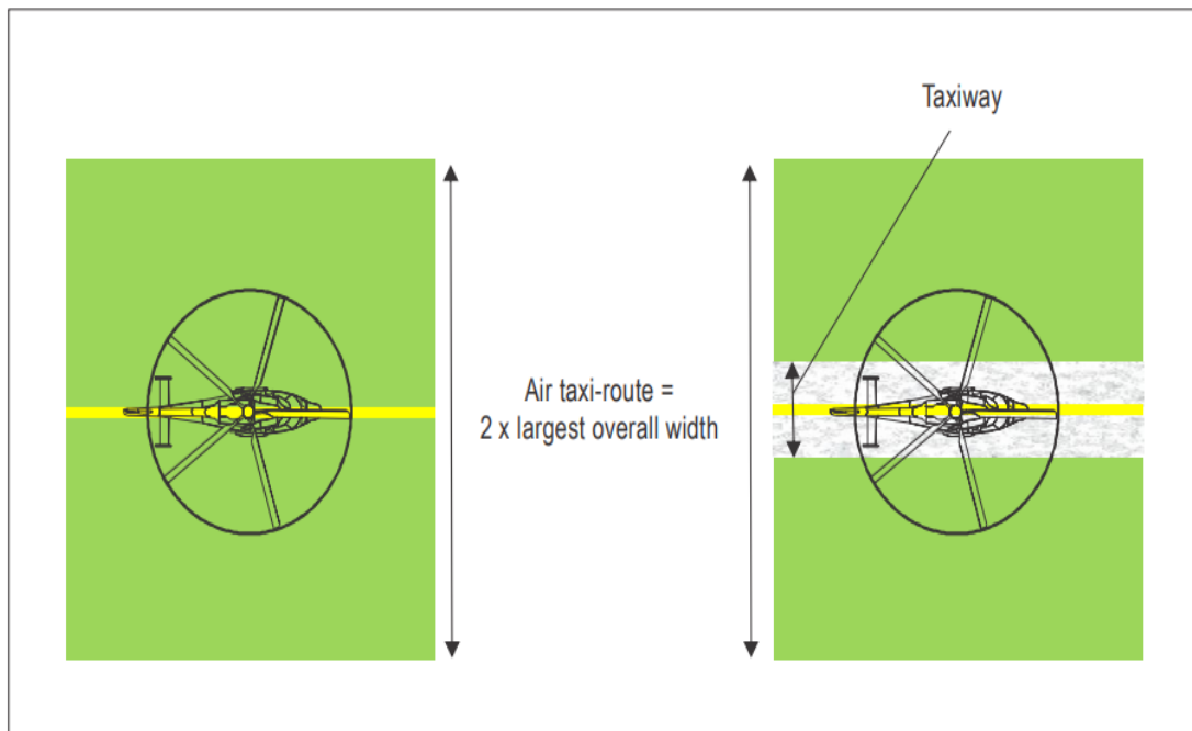
Figure 3-4. Helicopter air taxi-route and combined air taxi-route/taxiway
