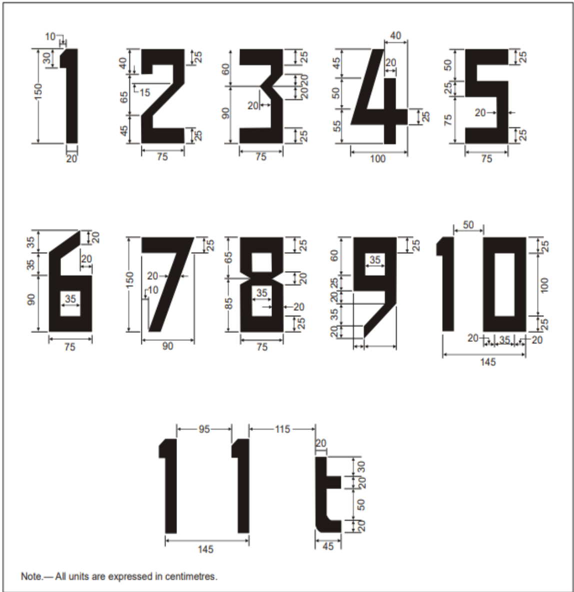
Figure 5-5. Form and proportions of numbers and letters
