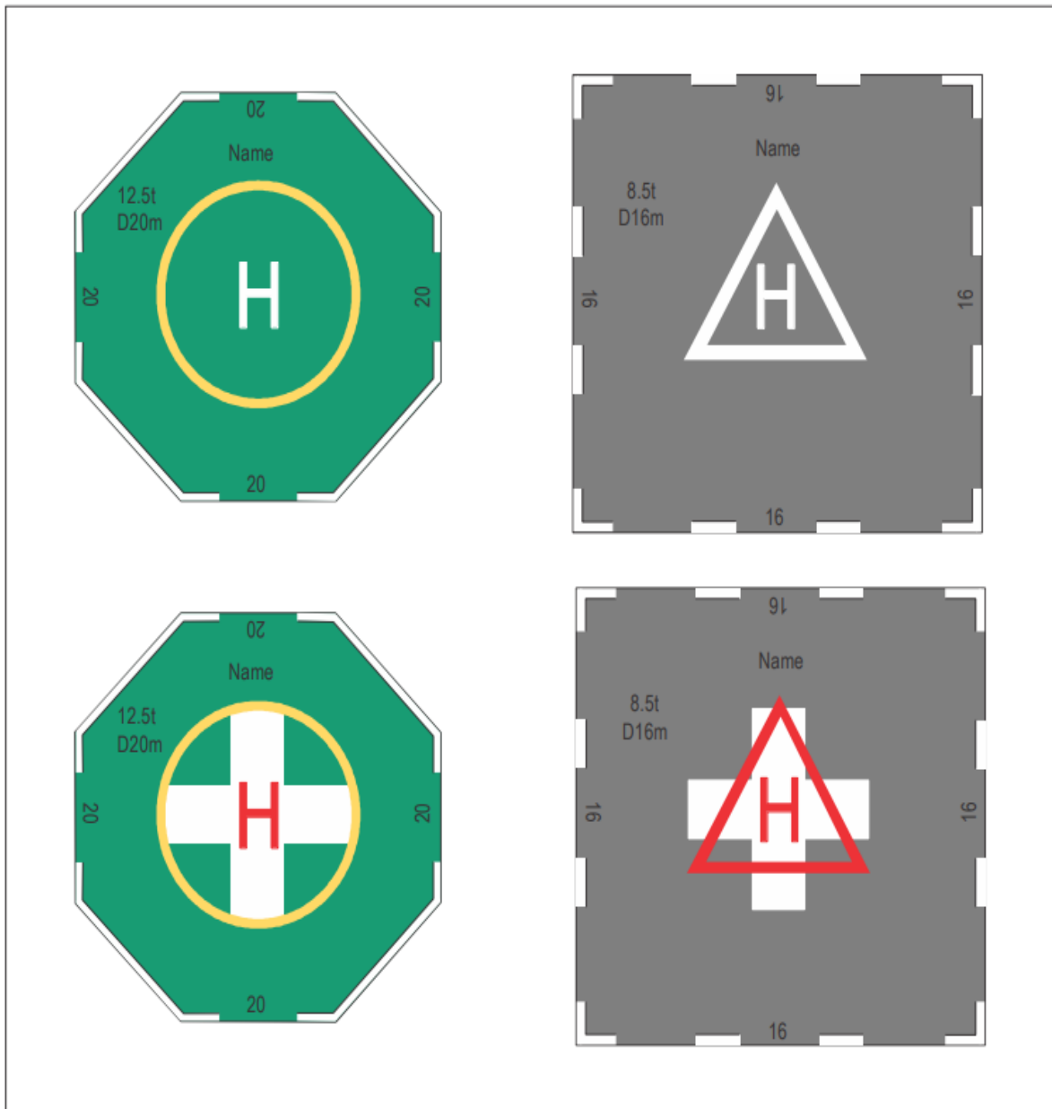
Figure 5-2. Heliport identification markings with TLOF and aiming markings for heliport and hospital heliport
