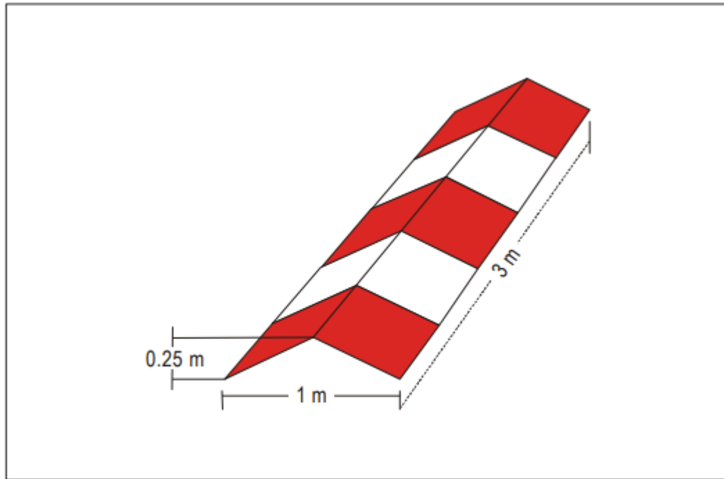
Figure 5-6. Runway-type FATO edge marker
