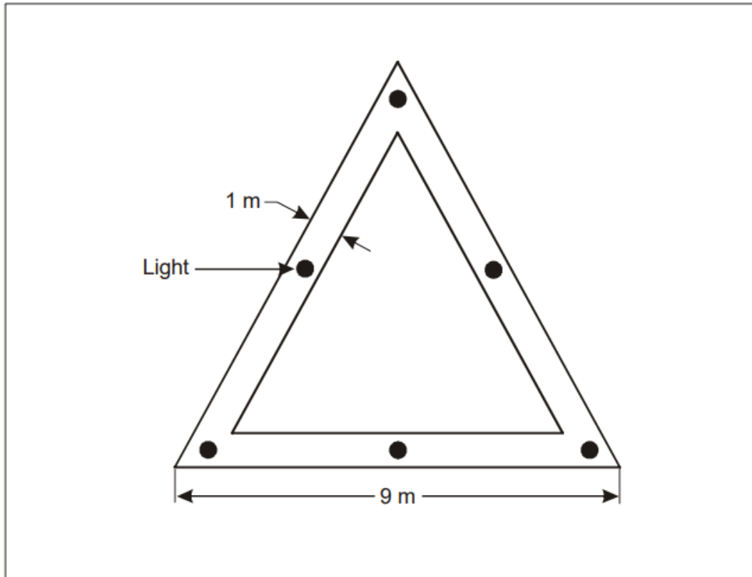
Figure 5-7. Aiming point marking
