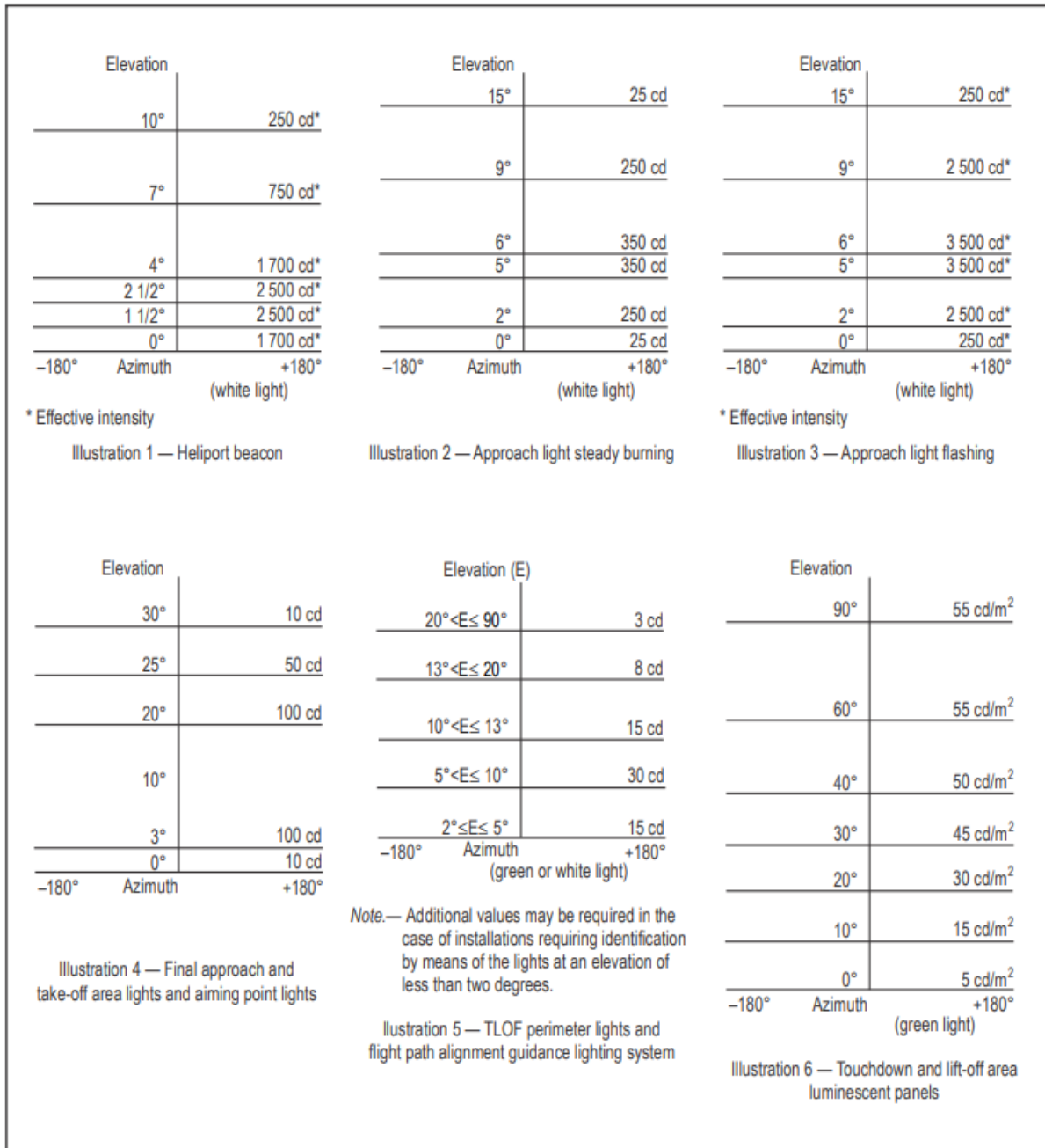
Figure 5-12. Isocandela diagrams
