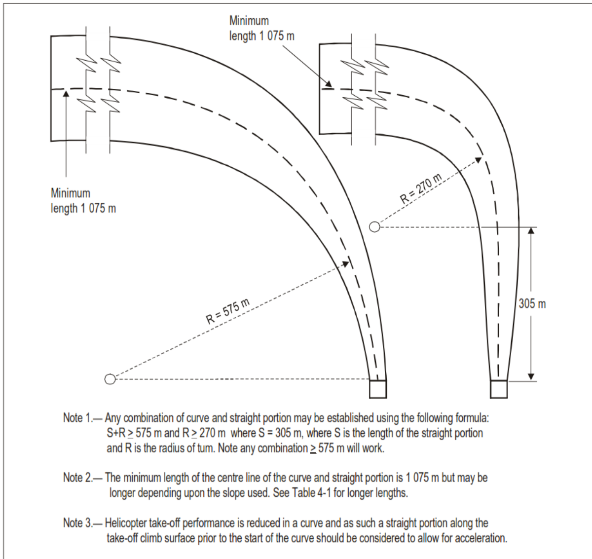
Figure 4-5. Curved approach and take-off climb surface for all FATOs
