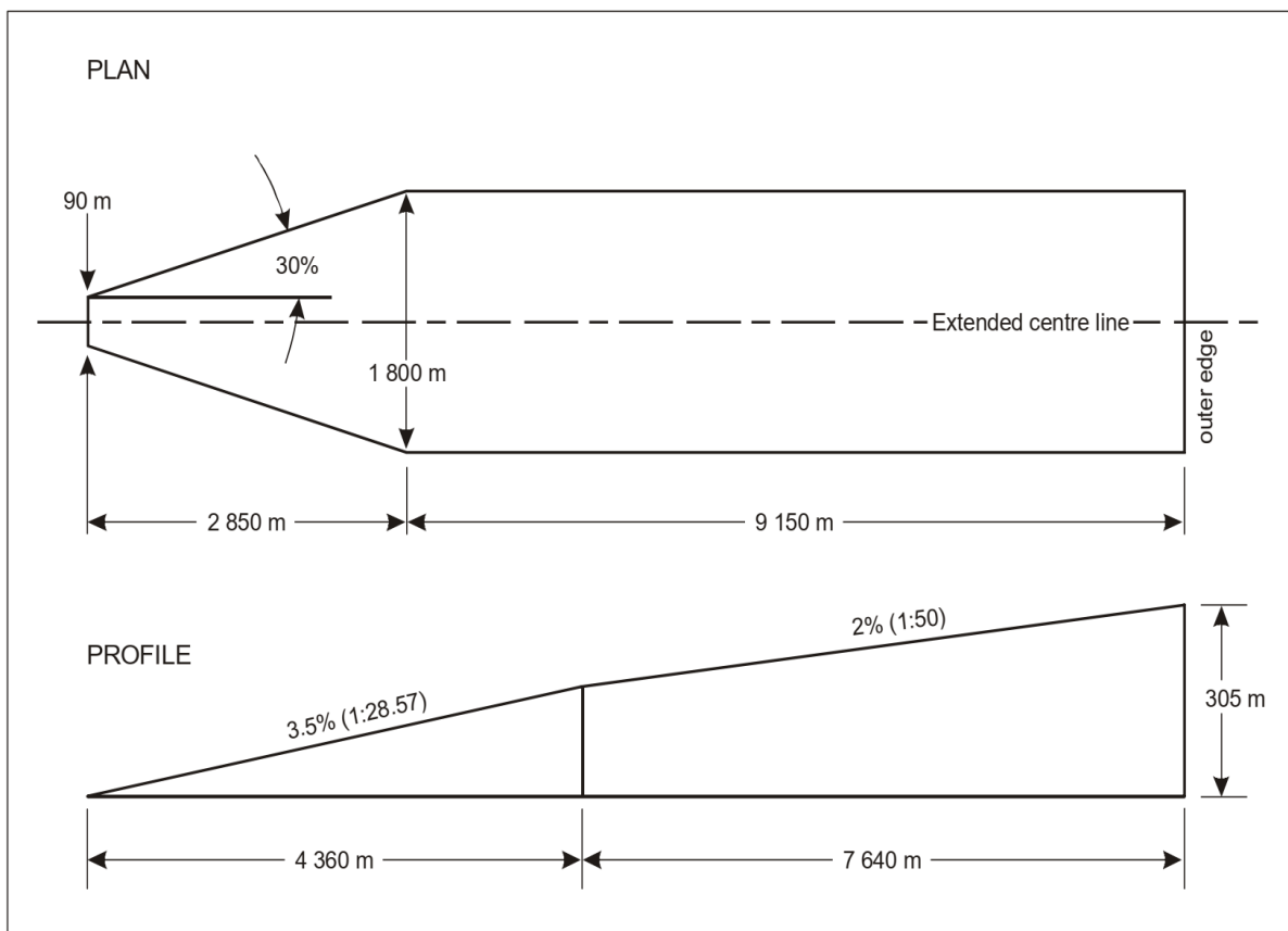
Figure A-2. Take-off climb surface for instrument FATO
