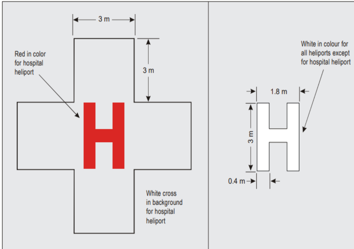
Figure 5-4. Hospital heliport identification and heliport identification marking
