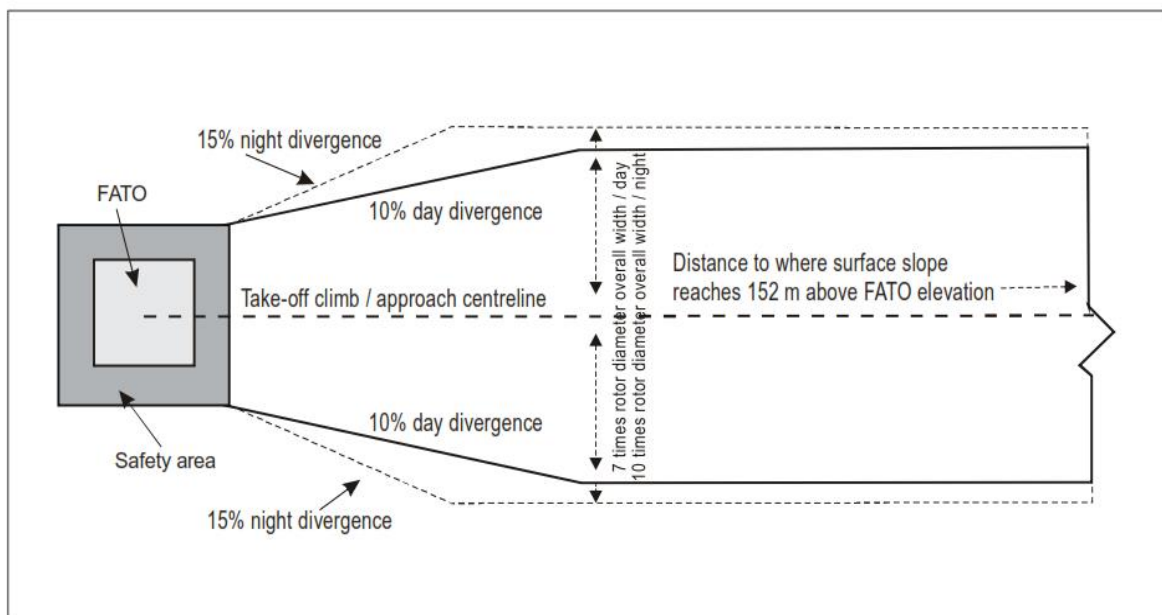
Figure 4-2. Take-off climb/Approach surface width
