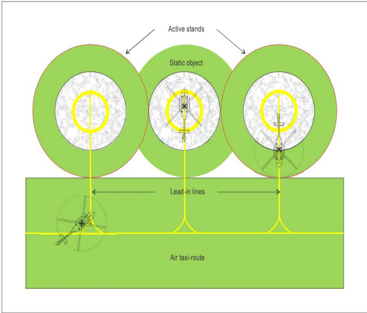
Figure 3-8. Turning stands (with air taxi-routes) non-simultaneous use — outer stands active
