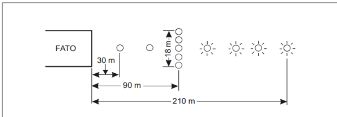
Figure 5-13. Approach lighting system
