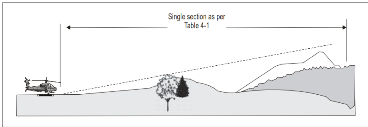
a) Approach and take-off climb surfaces - "A" slope profile - 4.5% design
