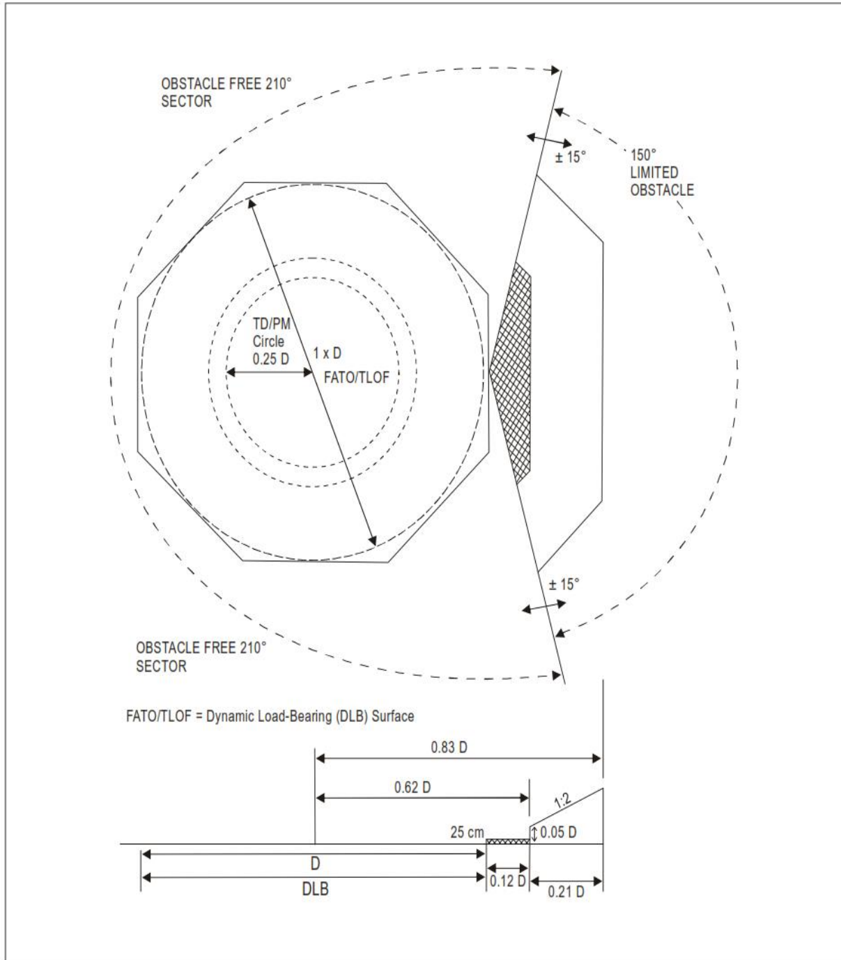
Figure 4-8. Helideck obstacle limitation sectors and surfaces for a FATO and coincidental TLOF of 1 D and larger
