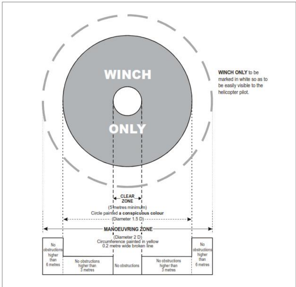
Figure 4-12. Winching area of a ship
