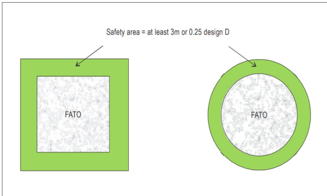
Figure 3-1. FATO and associated safety area
