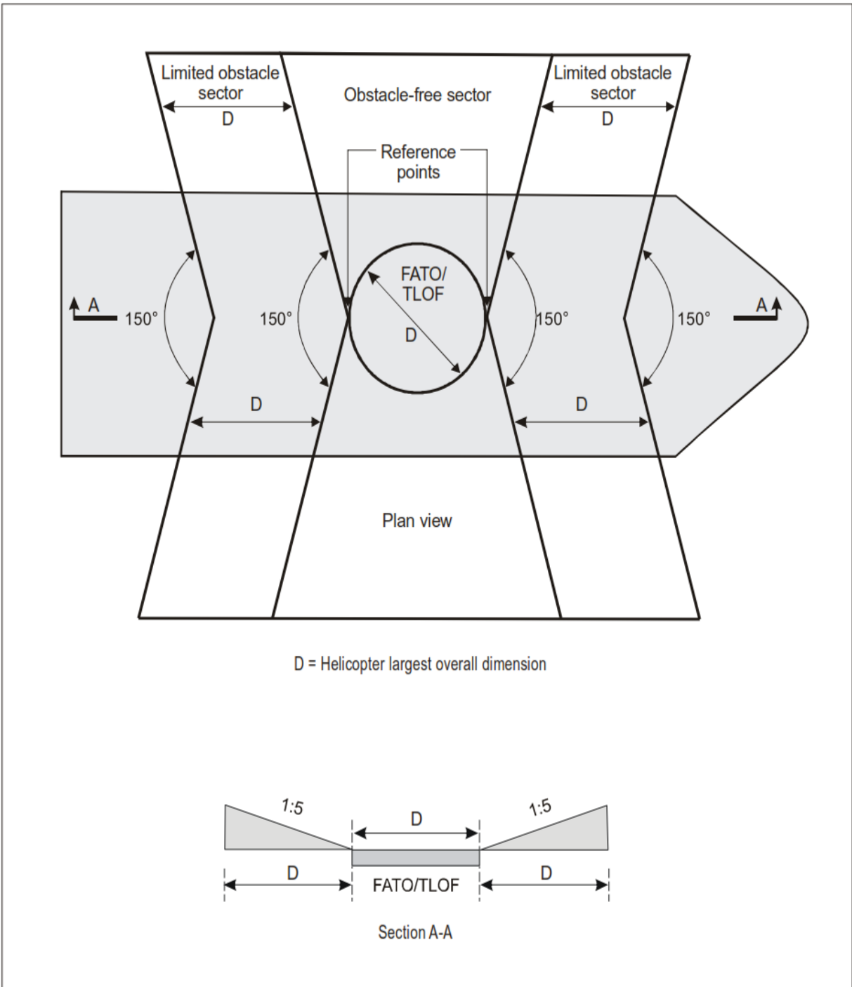
Figure 4-10. Amidship's location — Shipboard heliport obstacle limitation surfaces
