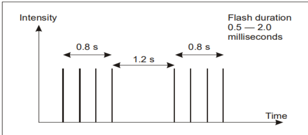
Figure 5-11. Heliport beacon flash characteristics
