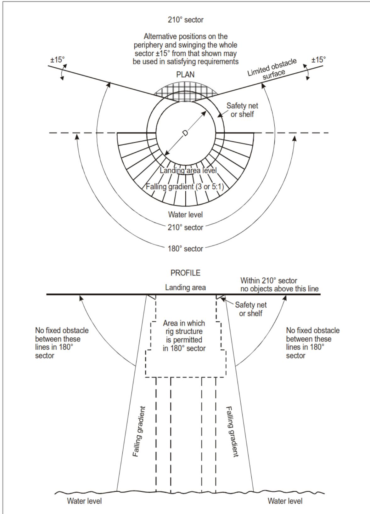
Figure 4-7. Helideck obstacle-free sector
