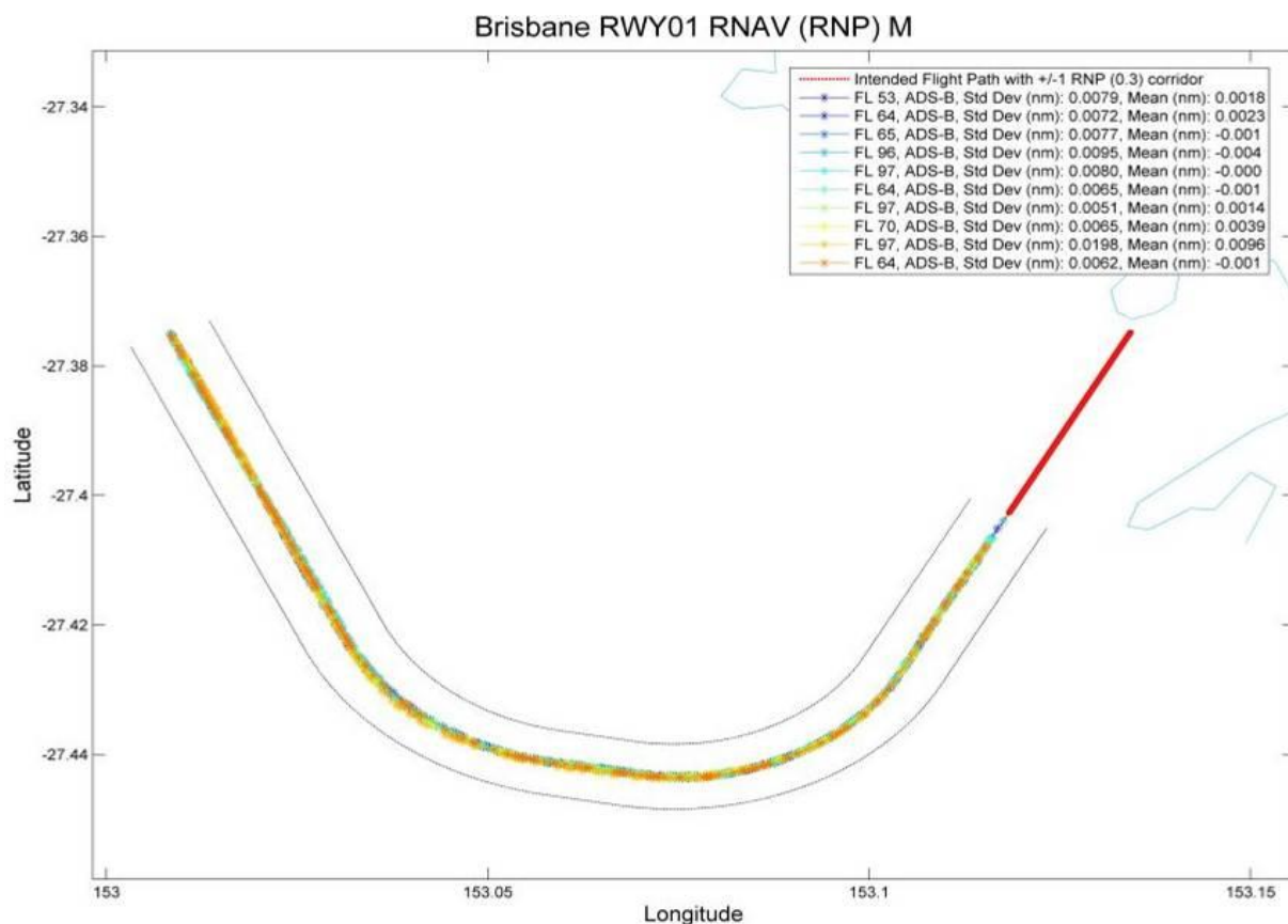
Figure 3.1: in-service data collected for RNP AR APCH operations
