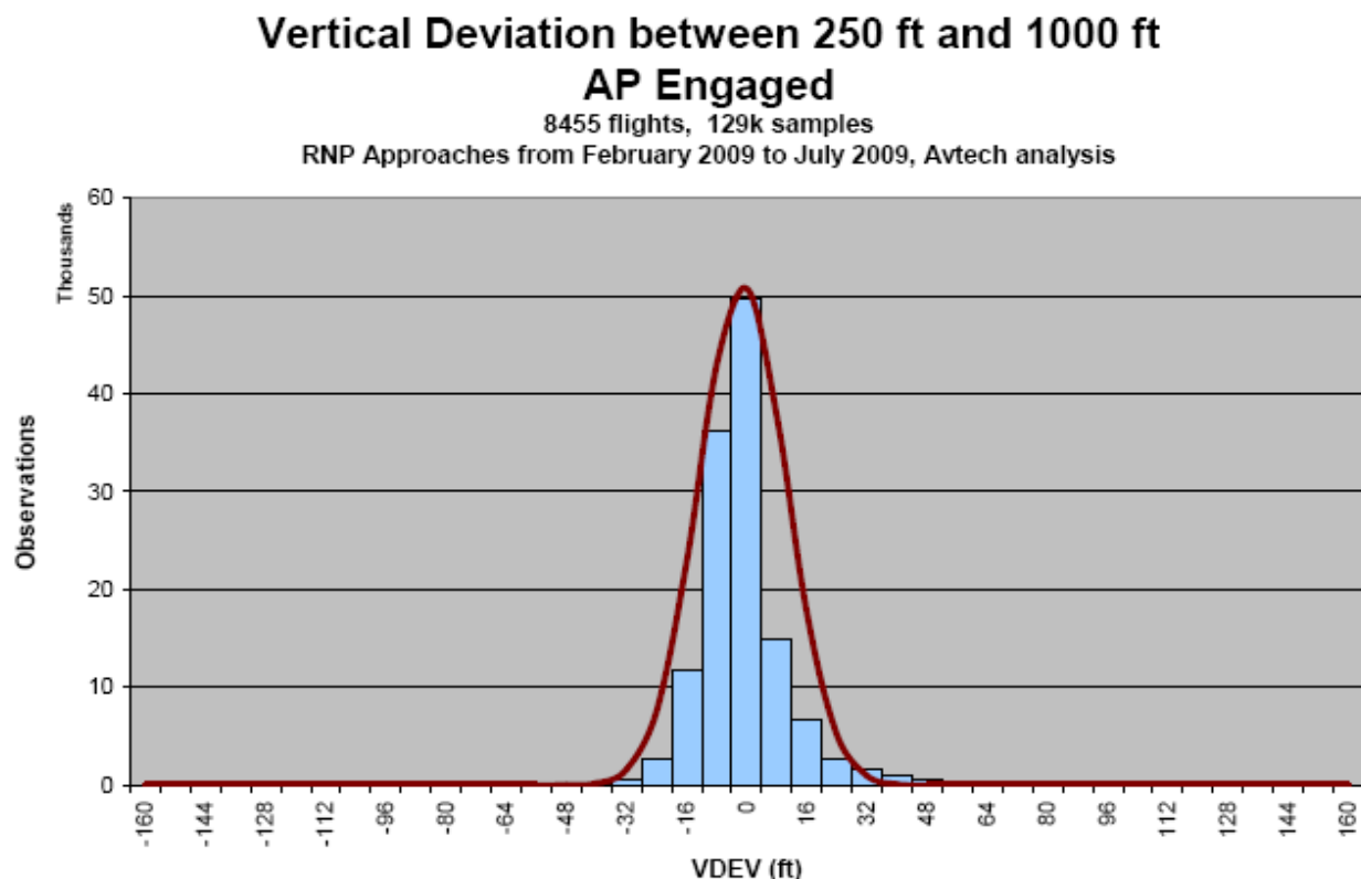
Figure 6.3: In-service Baro-VNAV FTE data
