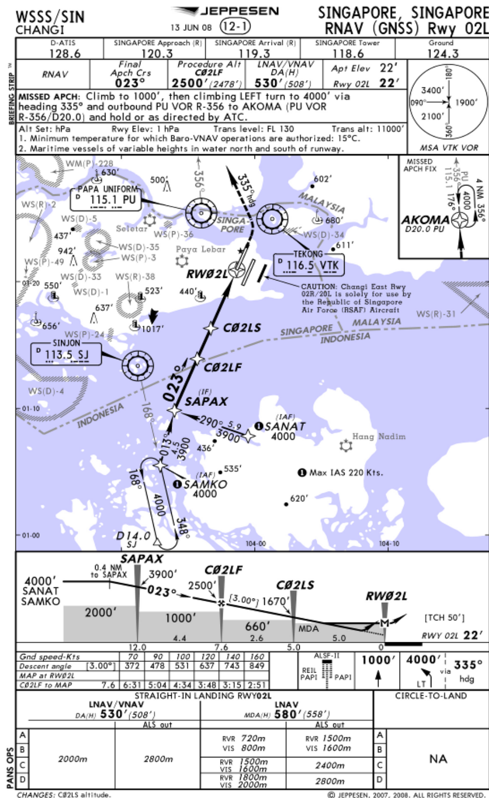
Figure 17.4 RNAV (GNSS) Approach Chart with LNAV and LNAV/VNAV Minima
