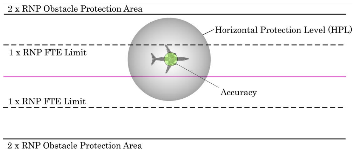
Figure 18.1: RNP AR APCH Obstacle Protection
