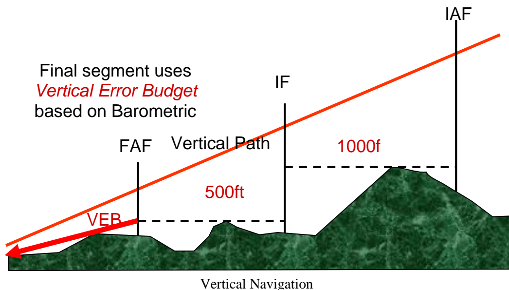
Figure RNP APCH
