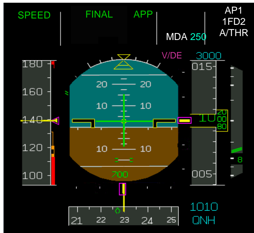
Figure 18.1: Primary Flight Display with lateral and vertical deviation indicators
