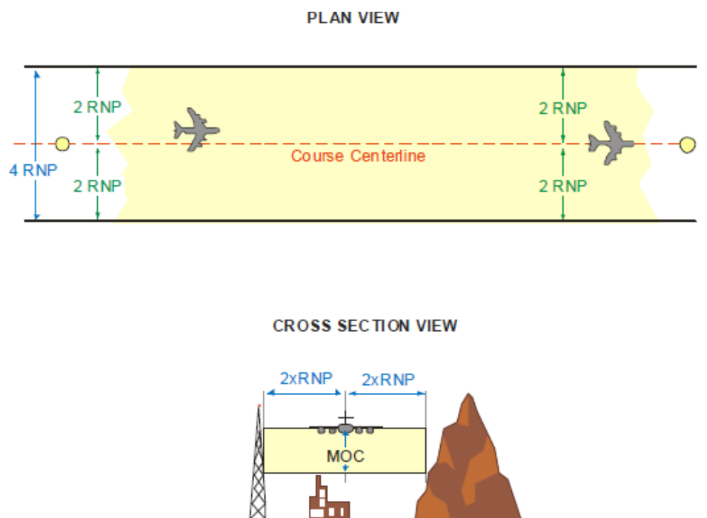
Figure 5.1 RNP AR APCH Obstacle Clearance
