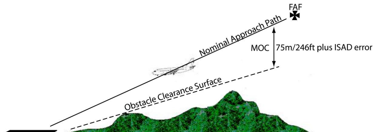
Figure 17.6: Baro-VNAV obstacle clearance for RNP APCH – LNAV
