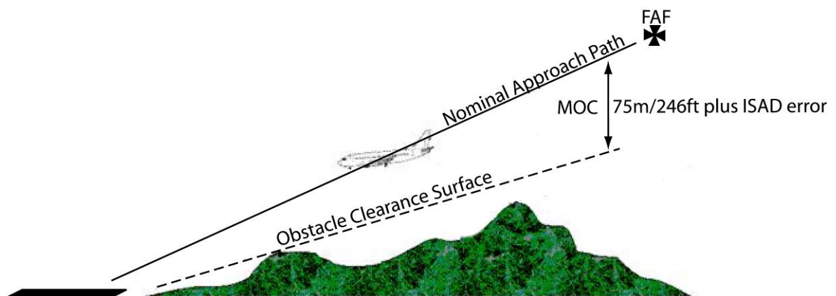
Figure 6.4: RNP APCH (LNAV/VNAV) Final Segment Obstacle Clearance
