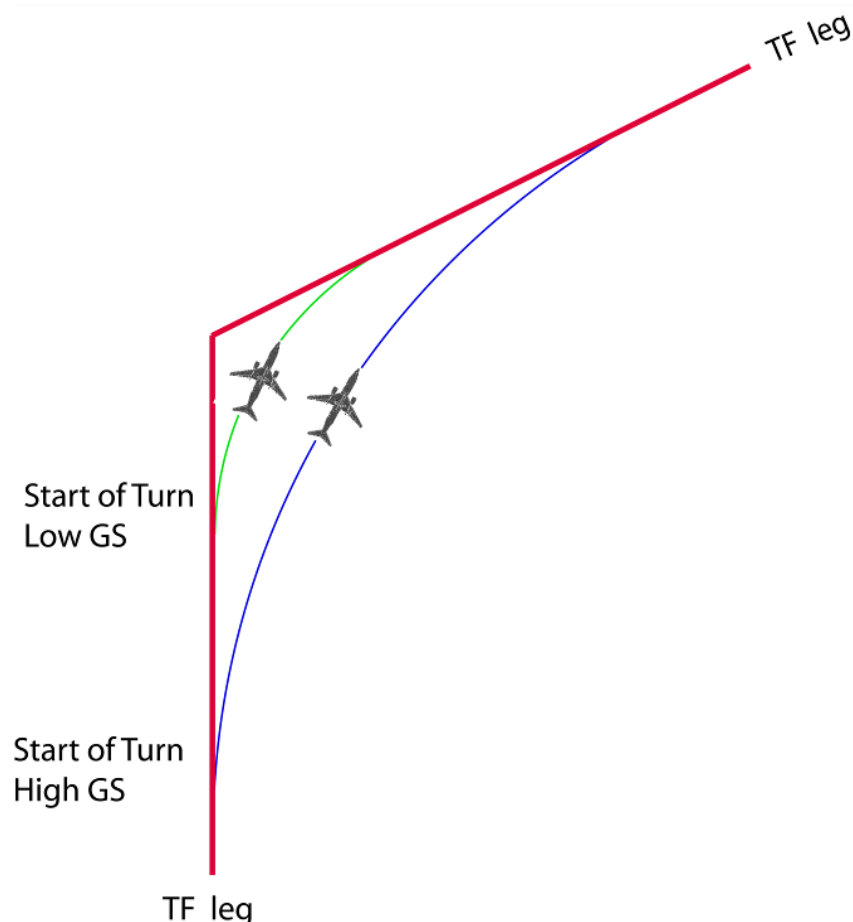
Figure 2.1: TF to TF Transition
