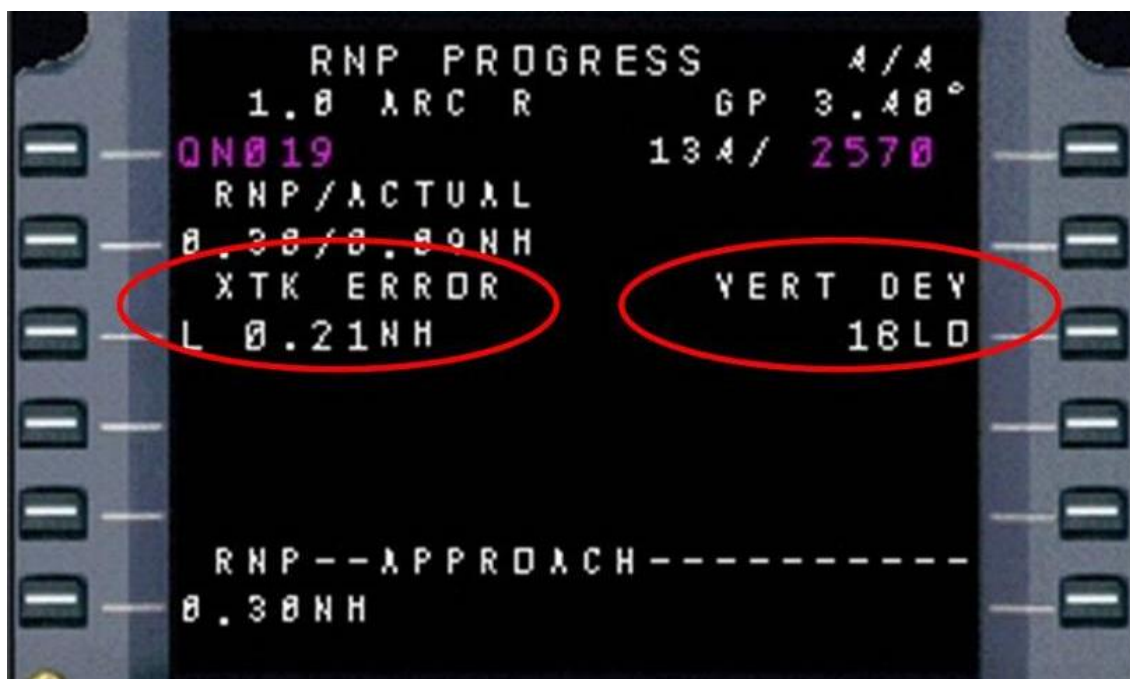
Figure 7.1: Cross-track and Vertical Deviations shown on Control and Display Unit
