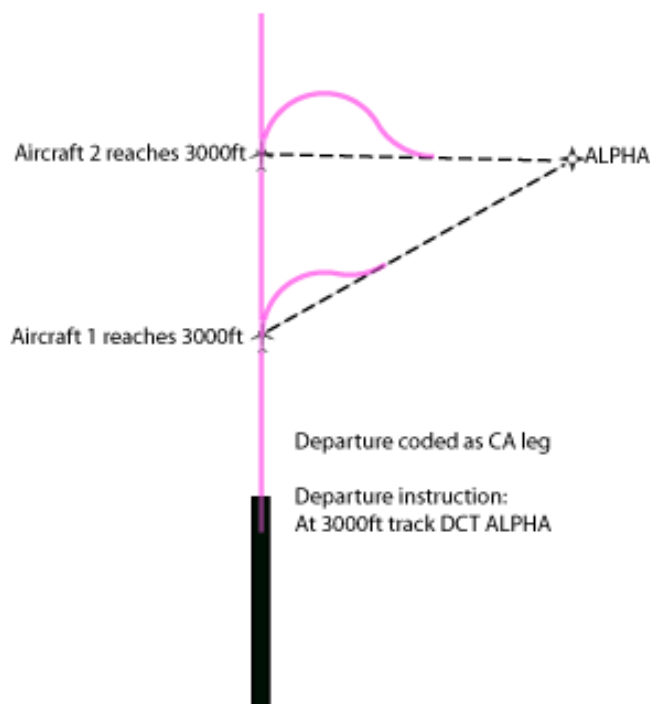
Figure 2.3: CA Path Terminator Example
