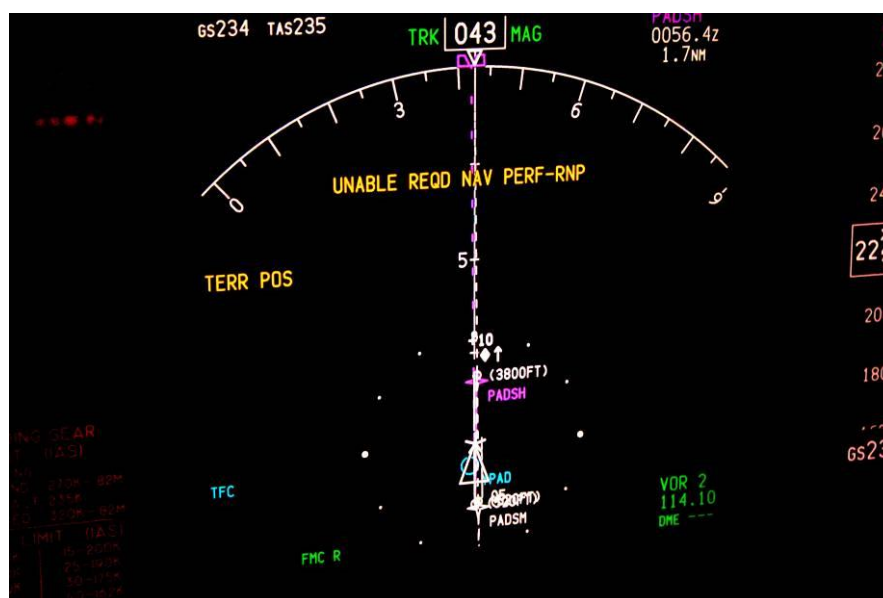
Figure 4.1: Alert annunciated on Boeing 737NG navigation display
