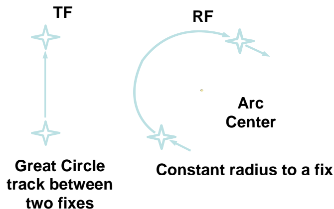
Figure 2.2: Common Path Terminators
